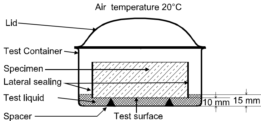
Fig. 1 Capillary suction.
