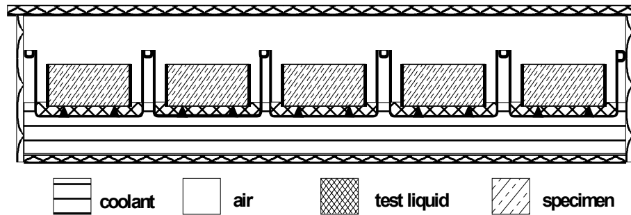
Fig. 3 Temperature controlled chest.
