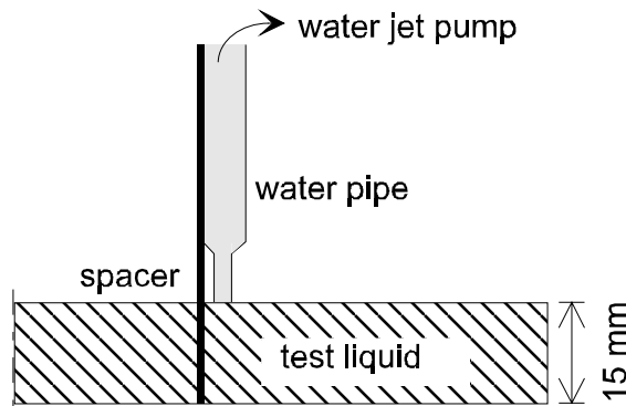
Fig. 5 Suction device to remove the liquid exceeding the level of 15 mm in the test containers.
