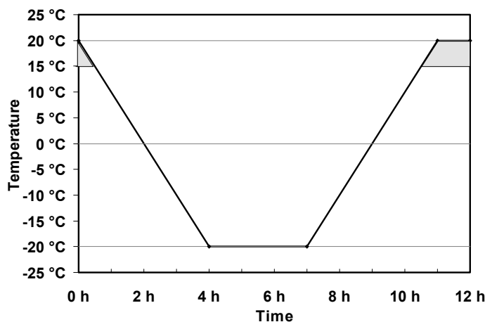
Fig. 6 Control temperature cycle.
