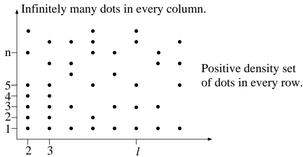
Figure 1: Schematic description of the proved cases of \mathrm{PSL}_2(\mathbb{F}_{\ell^n}) occurring as a Galois group over \mathbb{Q}
