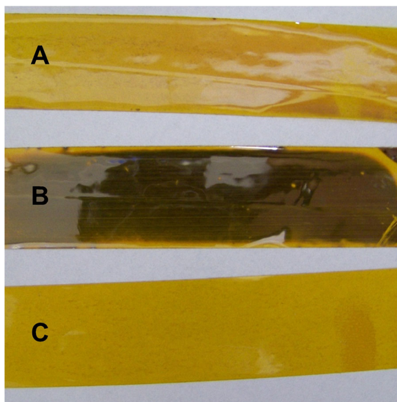
Fig. 8 Kapton tape stripes after the decomposition experiment of \text{Ag}(\text{hfacac})\text{PMe}_3 powder. a , b Tapes after experiment without and with ethanol, respectively. c Untreated reference tape
