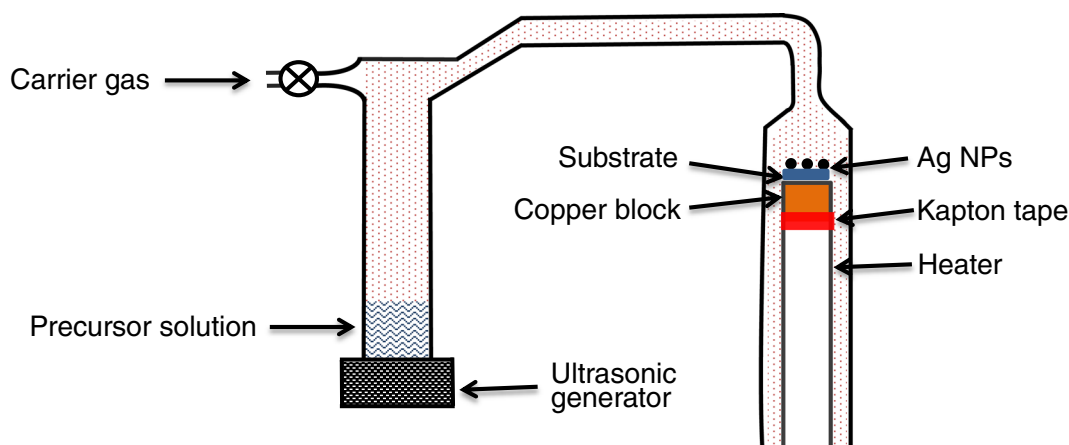
Fig. 1 Scheme of spray chemical vapour deposition set-up used for Ag NP film deposition
