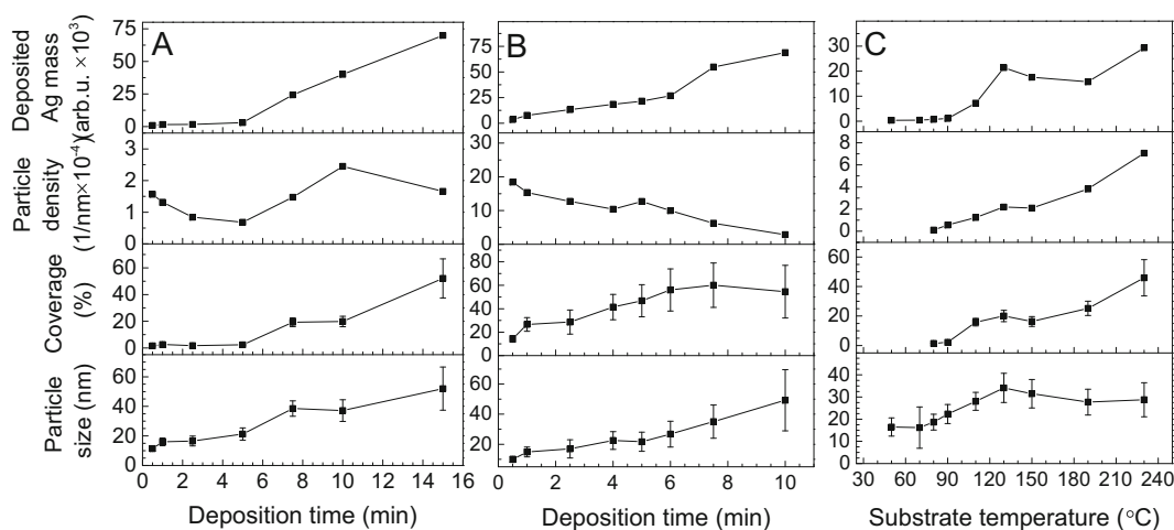
Fig. 4 Synoptic plots of crucial parameters of the obtained Ag NP films: deposited Ag mass, particle density, coverage and particle size. The error of deposited Ag mass is too small to visualize.
