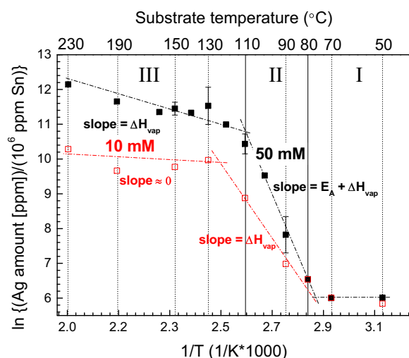
Fig. 7 Arrhenius plot of two series samples which were prepared with 10- and 50-mM precursor solution, respectively. Deposition time was 5 min for all the samples. Ag masses are relative values based on the internal standard Sn. The values of 90, 110, 130 and 150 °C samples were the average of two sample values, and the errors were obtained accordingly. The errors of other samples are too small to visualize
