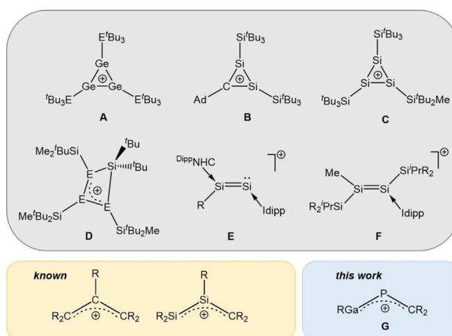
Scheme 1. Structurally characterized cations A–F ( E : R = I, H, Me, Et); F : R = Si( i -Pr)[CH(SiMe 3 ) 2 ]; A , D : E = Si, Ge) and resonance structures of allyl and heavier homologues.
