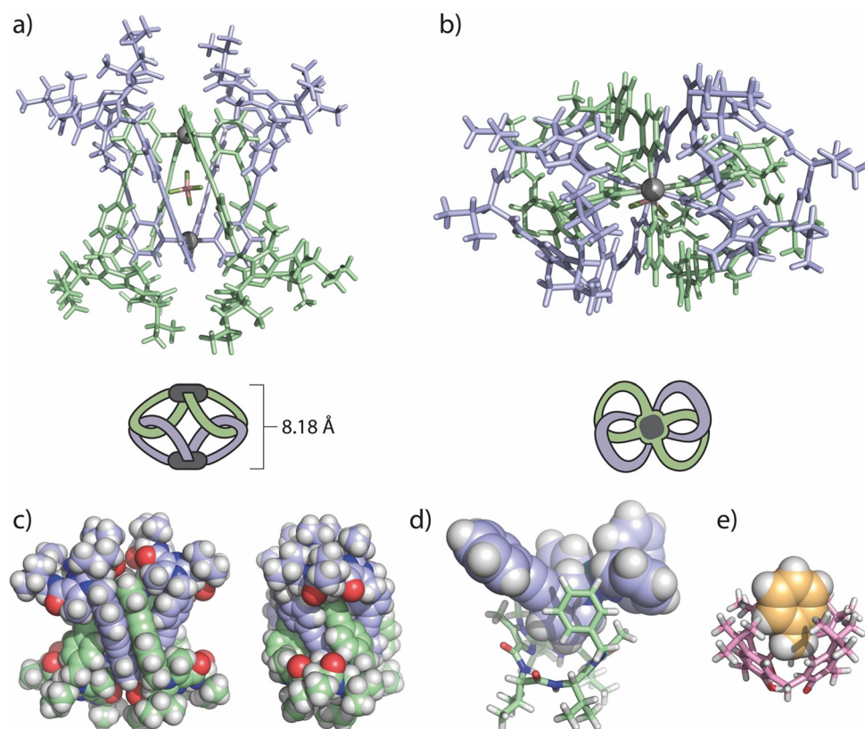
Figure 4. X-ray structure of [BF 4 @Pd 2 L 4 ](BF 4 ) (solvents and outer anions omitted for clarity): a) side and b) top view of the catenated motif; c) space filling side views; d) detail showing the non-covalent nesting of one of the coordinating pyridines in the basket-shaped macrocyclic backbone of another ligand and e) X-ray structure of toluene@calix-4-arene for comparison. [32]
