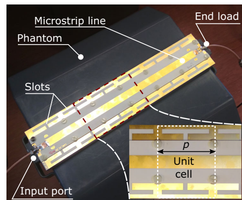
Fig. 8 Constructed prototype of leaky-wave antenna. Photographs of the fabricated prototype of the optimized LWA placed over a pelvis-shaped homogeneous phantom for MRI characterization.
