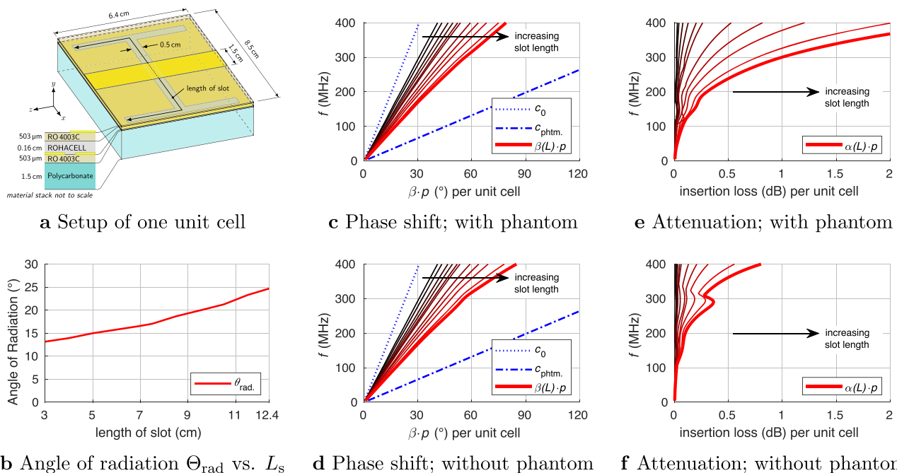
Fig. 4 A parametric numerical investigation of dispersion characteristics based on single unit cell. Geometry of the unit cell (a), angle \theta_{\text{rad}} of the leaky-wave radiation for the loaded transmission line (b), phase shift ( \beta \cdot p ) and insertion loss (dB) ( \alpha \cdot p \cdot 20 \log(10)^{-1} ) in the microstrip leaky-wave transmission line per unit cell (c, d–f). The length of the slot is varied from 3 cm to 12.4 cm. In cases c, e, the transmission line is placed on a phantom while cases d, f represent the free space environment of the transmission line. The bold curves are for the LWA with an optimal length of 12.4 cm.
