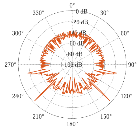
FIGURE 34. PRT-simulated relative backscatter power of a full 3D mite model recorded in a monostatic geometry for different rotation angles at 300 GHz (Scenario I).
