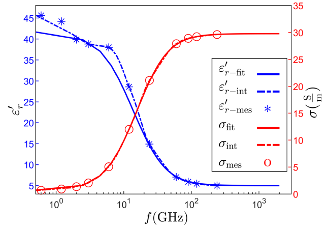
FIGURE 28. The retrieved dielectric function showing the Debye model of the permittivity (solid blue line), the interpolated measured permittivity (dash-dotted blue line), the Debye model of the conductivity (solid red line), and the interpolated measured conductivity (dash-dotted red line). The fitted conductivity is very close to the interpolated measured conductivity and hence the red dash-dotted line is hardly visible. The markers depict the available experimental data [62].
