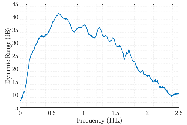
FIGURE 20. Dynamic range of the employed setup, calculated by subtracting a measurement without any sample and a measurement without any sample and a measurement against a metal plate as a reference measurement.
