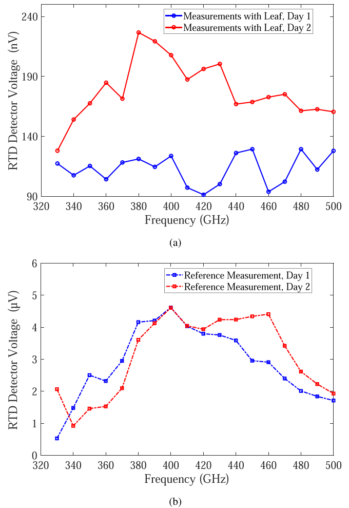
FIGURE 3. (a) The voltage recorded from the RTD detector during two consecutive days of measurements of a Geranium leaf. (b) The voltage was recorded from the RTD detector during two consecutive days of measurements without leaf (reference measurements).
