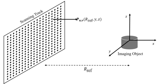
FIGURE 9. 3D SAR imaging geometry.
