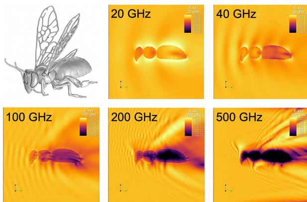
FIGURE 31. 3D-FDTD simulation of the electric field's absolute value for a plane wave illumination from the left (y-direction). The field distribution displays the penetration behavior into the volumetric bee model at different frequencies between 20–500 GHz.
