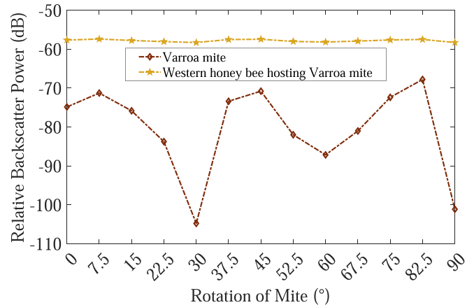
FIGURE 35. Relative backscatter power for 13 rotation steps (Scenario II) of a full 3D mite model in its initial position.
