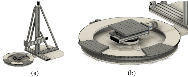
FIGURE 8. Future cylindrical positioning system offering extended scanning capabilities including bi-static RCS and along-the-stem axis measurements.
