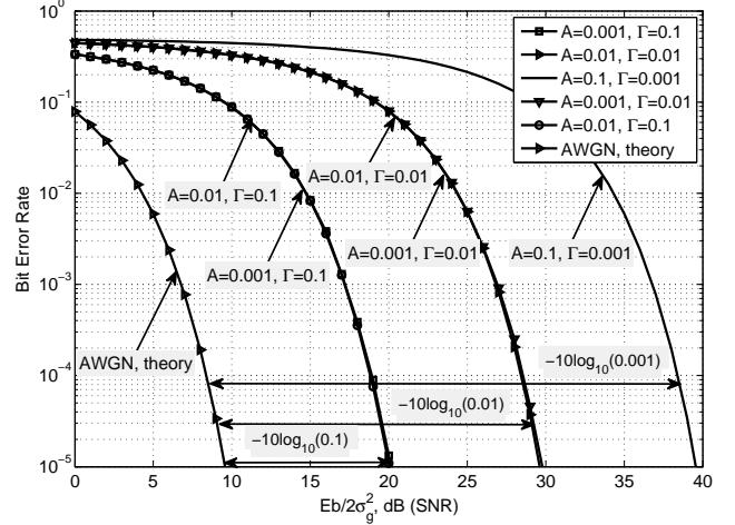
Figure 10: Shows that with MC modulation the SNR requirement is \sigma_I^2 = 1/\Gamma instead of 1/A\Gamma , even though a symbol is affected by impulse noise of variance \sigma_I^2/A . BPSK OFDM was used, with a DFT size of 10000.
