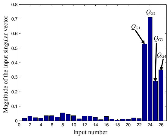
Figure 9: Input singular vector associated with inter-area mode
