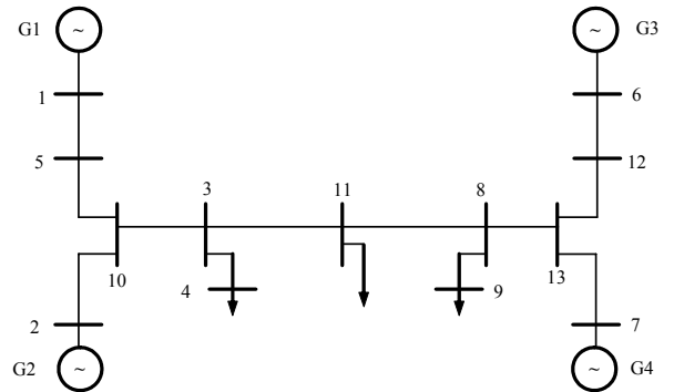
Figure 2: Four-machine two-area power system model
