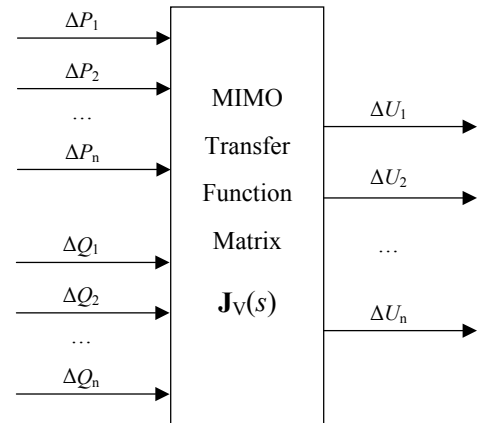
Figure 1: Dynamic voltage stability modeling
