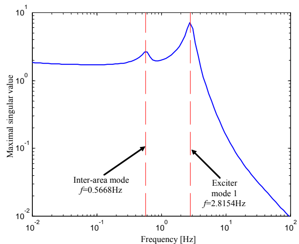
Figure 5: Maximal singular value plot
