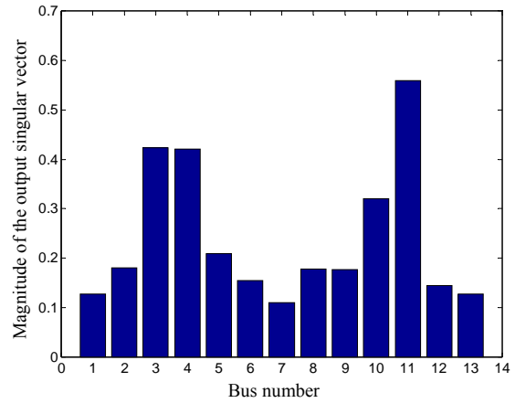
Figure 8: Output singular vector associated with inter-area mode
