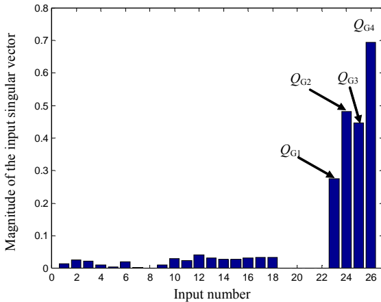
Figure 7: Input singular vector associated with exciter mode 1
