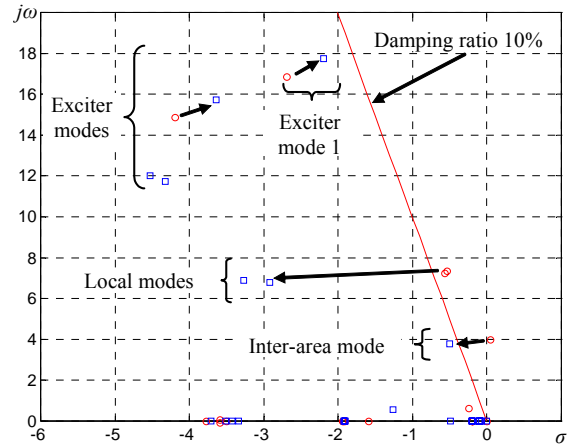
Figure 4: Critical eigenvalues of the power system
