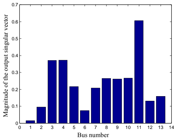
Figure 10: Output singular vector of the transfer function matrix J_V(s) when s=0
