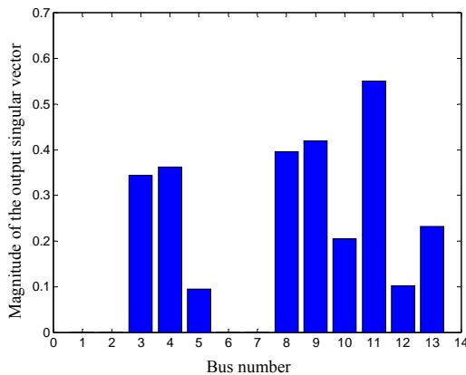
Figure 3: Output singular vector plot for the static voltage stability analysis
