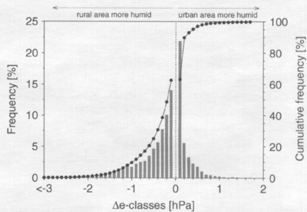
Figure 4. Frequency (grey bars) and cumulative frequency (circles) distribution of urban/rural water vapour pressure differences ( \Delta e_{u-r} ) in Krefeld (11/2001–10/2002, based on hourly averages). This figure is available in colour online at www.interscience.wiley.com/ijoc
