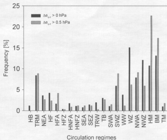
Figure 6. Correlation of UME data versus European 'Grosswetterlagen' as classified by Gerstengarbe and Werner (1999). Zonal circulation patterns: westerly type, cyclonic (WZ); angular westerly type (WW) Mixed circulation patterns: southwesterly type, anticyclonic (SWA); southwesterly type, cyclonic (SWZ); northwesterly type, anticyclonic (NWA); northwesterly type, cyclonic (NWZ); high, Central Europe (HM); ridge of high pressure, Central Europe (BM); low, Central Europe (TM) Meridional circulation patterns: high, British Islands (HB); trough, Central Europe (TRM); northeasterly type, anticyclonic (NEA); high, Fennoscandia, anticyclonic (HFA); high, Fennoscandia, cyclonic (HFZ); high, Arctic Ocean–Fennoscandia, anticyclonic (HNFA); high, Arctic Ocean–Fennoscandia, cyclonic (HNFZ); southeasterly type, anticyclonic (SEA); southeasterly type, cyclonic (SEZ); Low, British Islands (TB); trough, Western Europe (TRW).
