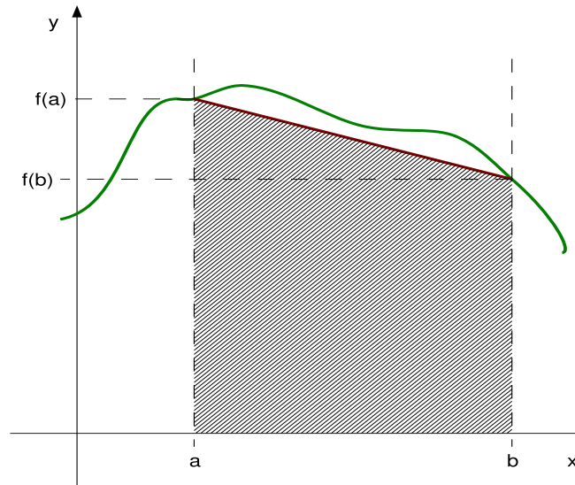
Trapezoidal rule
