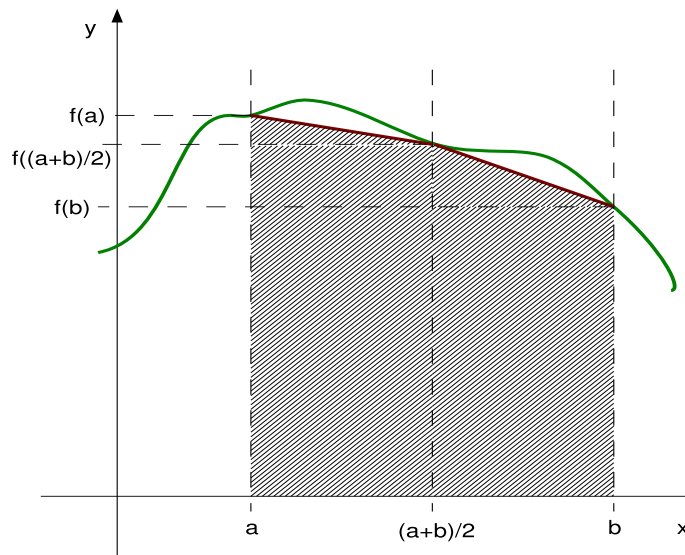
composite Trapezoidal rule for n=2
