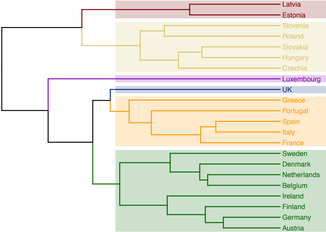
Figure 2: Result of the hierarchical clustering.
