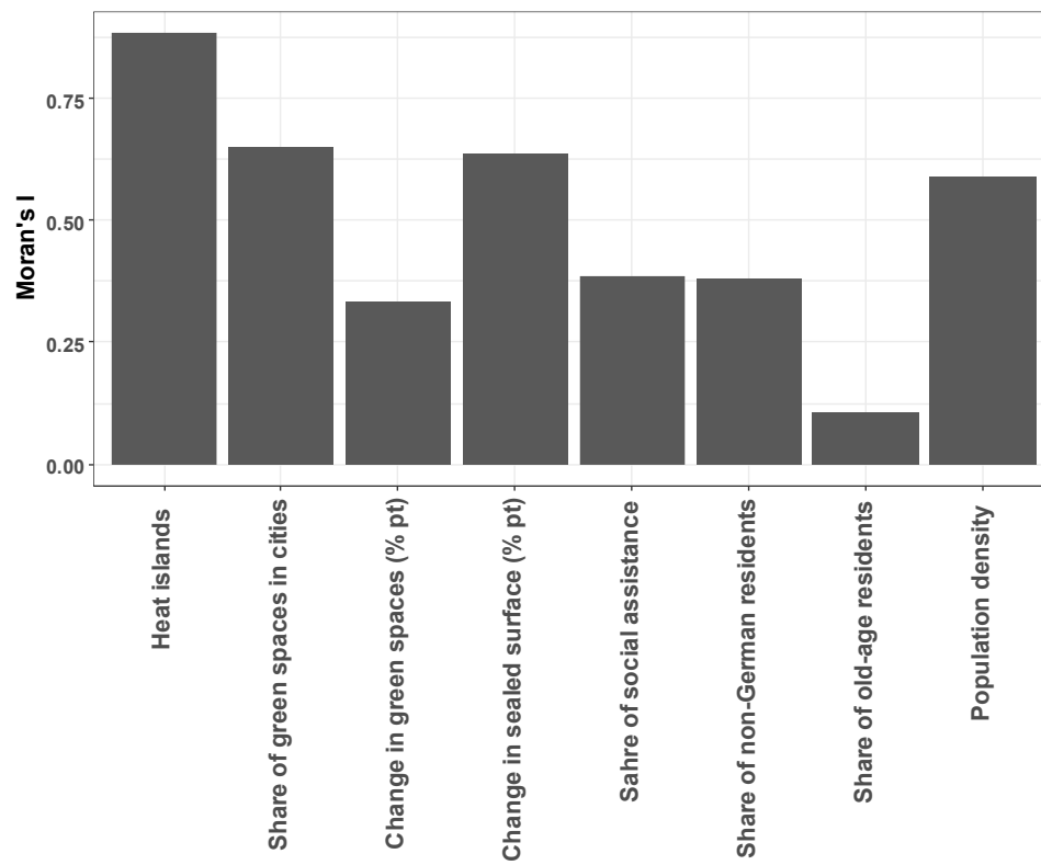
Figure A6: Moran's I statistic for key variables.
