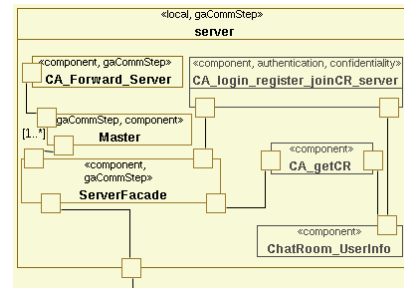
Figure 10. Alternative implementable architecture
