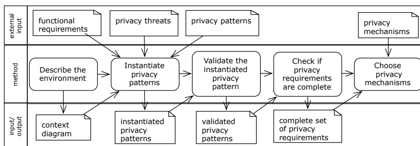
Fig. 2. A Method for Using Privacy Patterns
