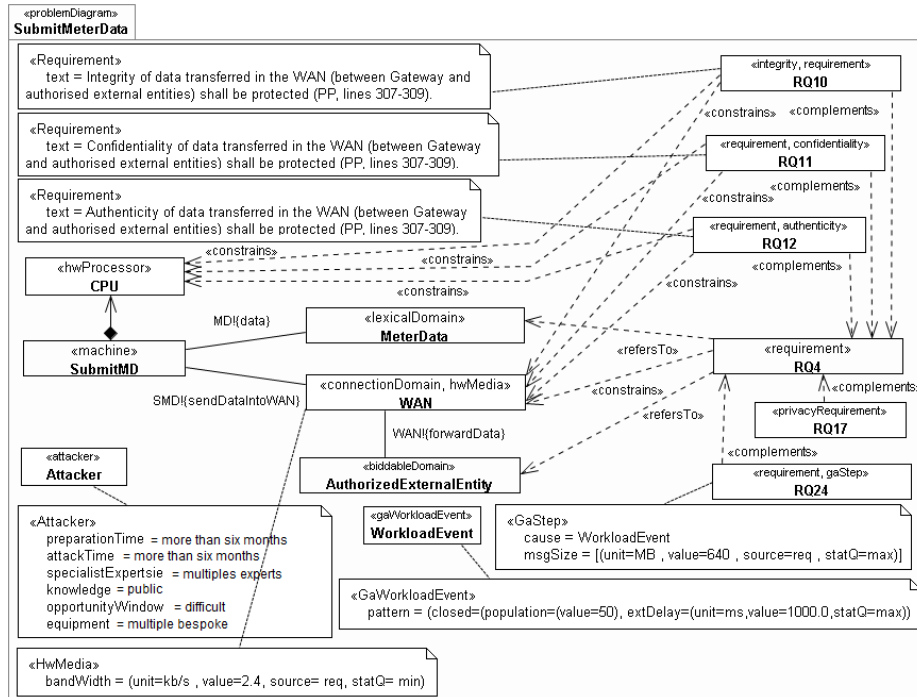
Fig. 2. Problem Diagram for submitting meter data to external entities
