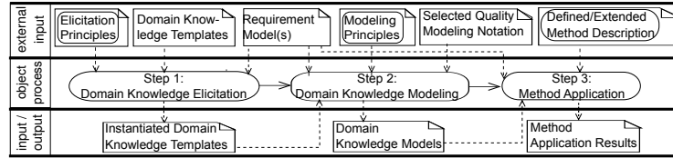
Fig. 5. Object-process for eliciting, modeling, and using domain knowledge
