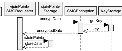
Fig. 8. Sequence diagram for aspect R32
