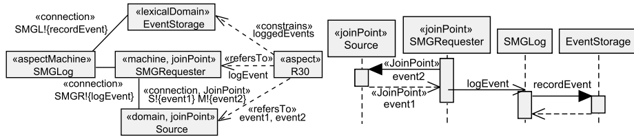
Fig. 6. Sequence diagram for aspect R30
