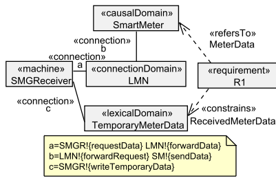
Fig. 3. Problem Diagram for R1
