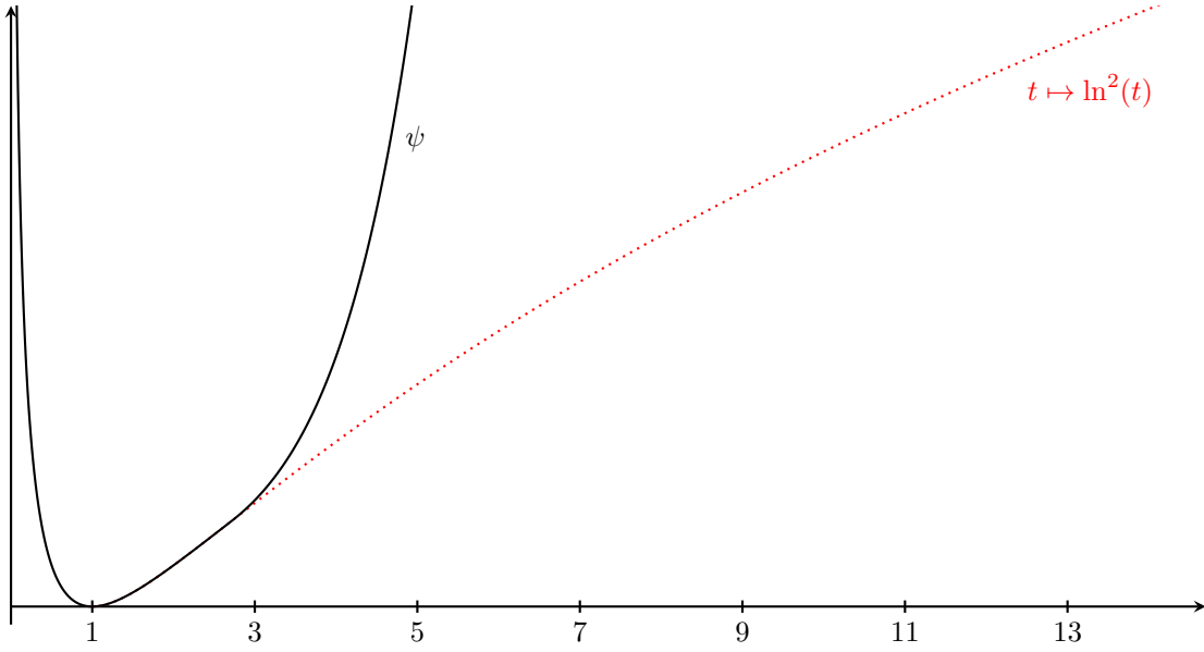
Figure 3: The volumetric part \psi of the polyconvex extension and the original volumetric term \ln^2(t) of the classical Hencky energy.
