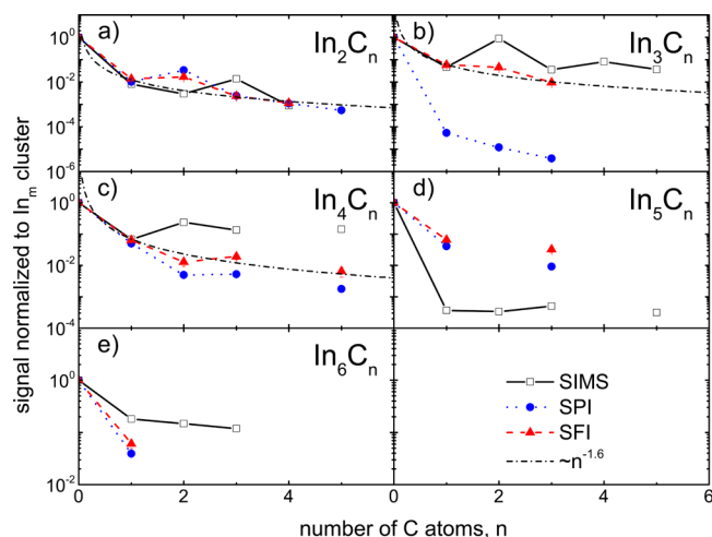
Figure 5. Size distribution of neutral (SPI, blue; SFI, red) and ionized (SIMS, black) \text{In}_m\text{C}_n clusters containing a fixed number of indium atoms produced under bombardment of solid indium with 20 keV \text{C}_{60}^+ ions. The signals were normalized to that of the respective \text{In}_m cluster.
