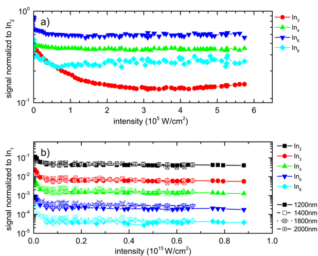
Figure 3. Signal of postionized neutral indium atoms and clusters produced under bombardment of solid indium with 20 keV C 60 + ions normalized to that of In 2 dimers (a) or In atoms (b) vs ionization laser intensity for (a) VUV single photon ionization at 157 nm and (b) IR strong field photoionization at the indicated wavelength.
