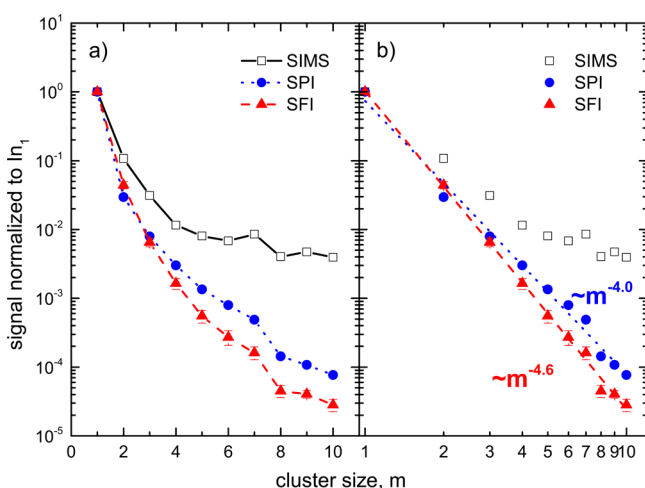
Figure 4. Size distribution of neutral In m clusters (SFI, red) and In m + cluster ions (SIMS, black) produced under bombardment of a solid indium surface with 20 keV C 60 + ions plotted in (a) semilog and (b) double-log fashion. The neutral species were postionized using either a VUV single photon ionization (SPI, blue) or a IR strong field photoionization (SFI, red) scheme.
